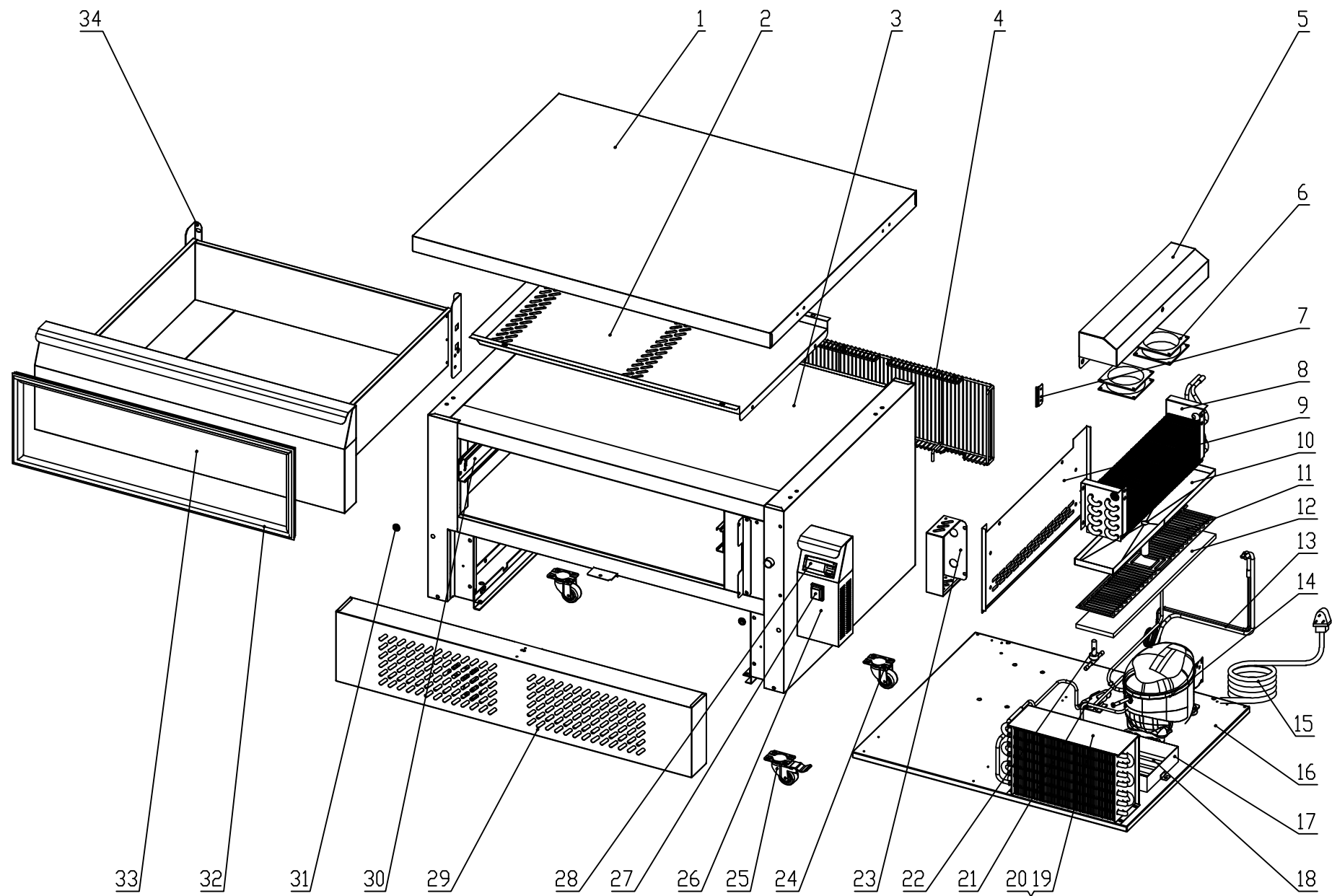
EXPLODE OF CBR1-2/CBR1-3
