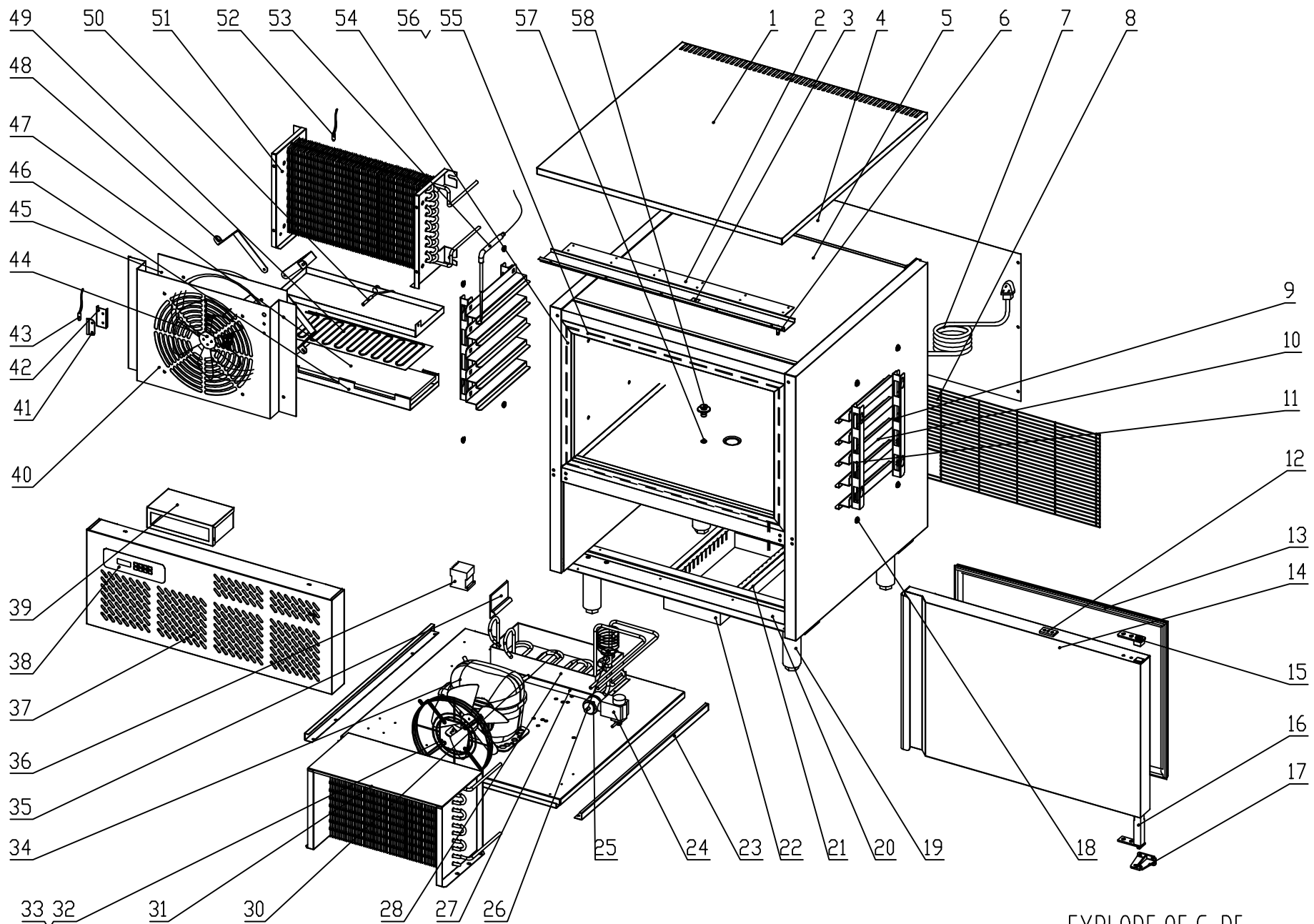
EXPLODE OF G-D5
