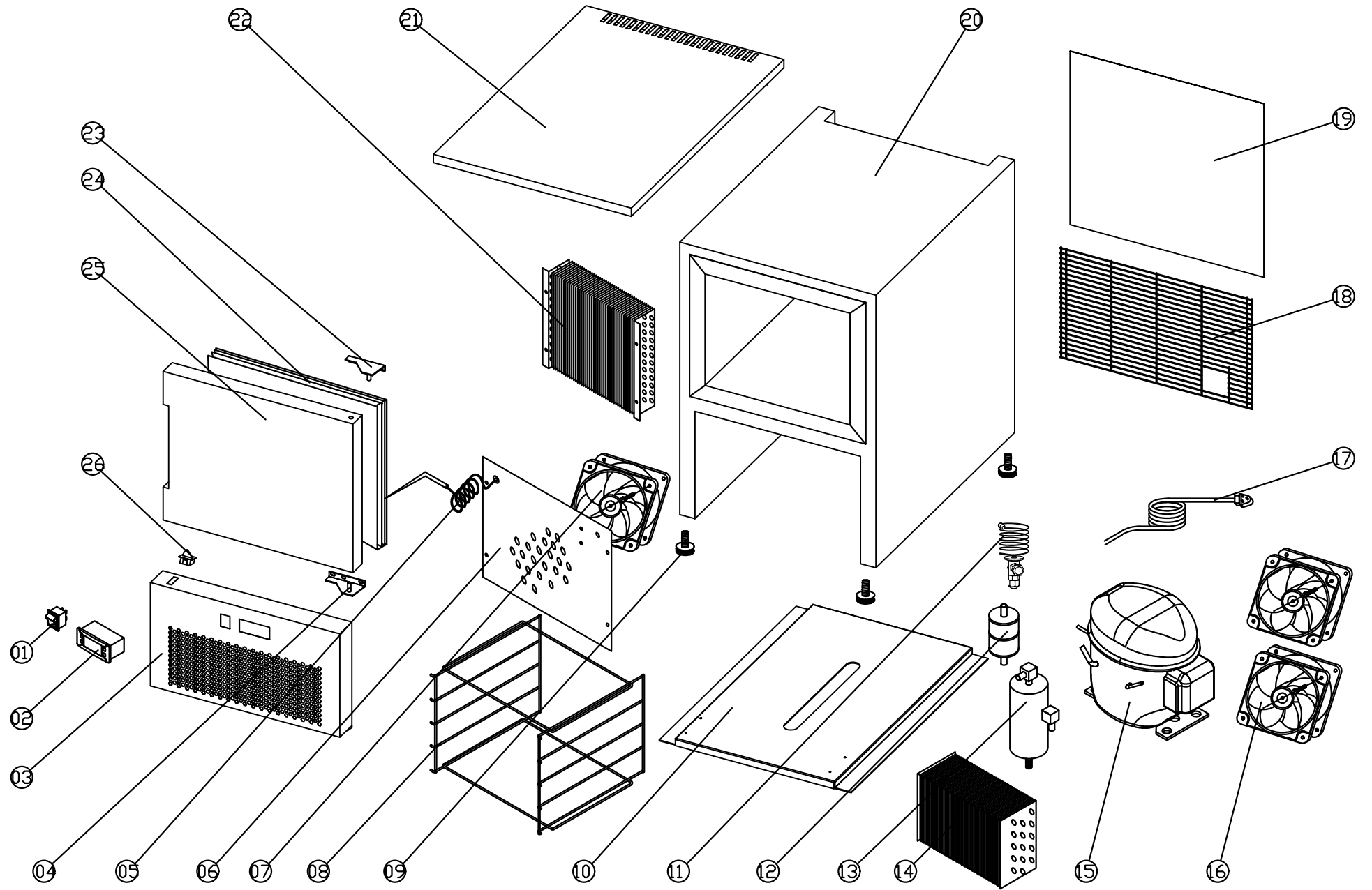
EXPLODE DIAGRAM OF DT3
